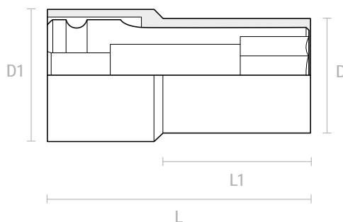
Nástrčná hlavice Surface-drive 1", Pinch-point Socket surface-drive 1", Pinch-point
