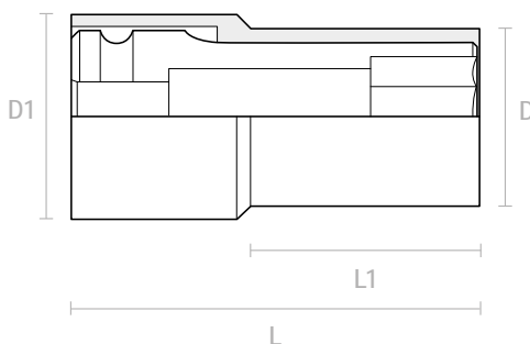
Nástrčná hlavice 6-ti hranná 1", Pinch-point 6-point socket 1", Pinch-point
